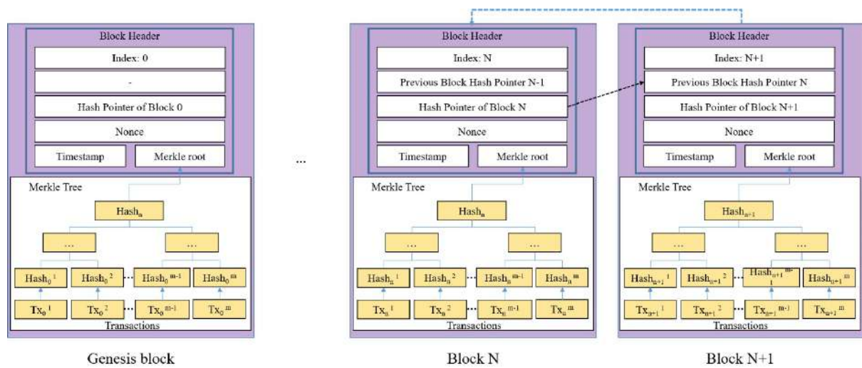
Fig. 1. An example of a blockchain
