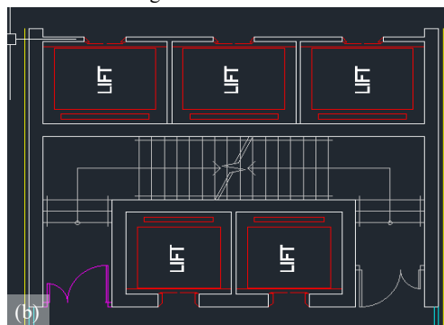
As-designed data 2D CAD drawings
