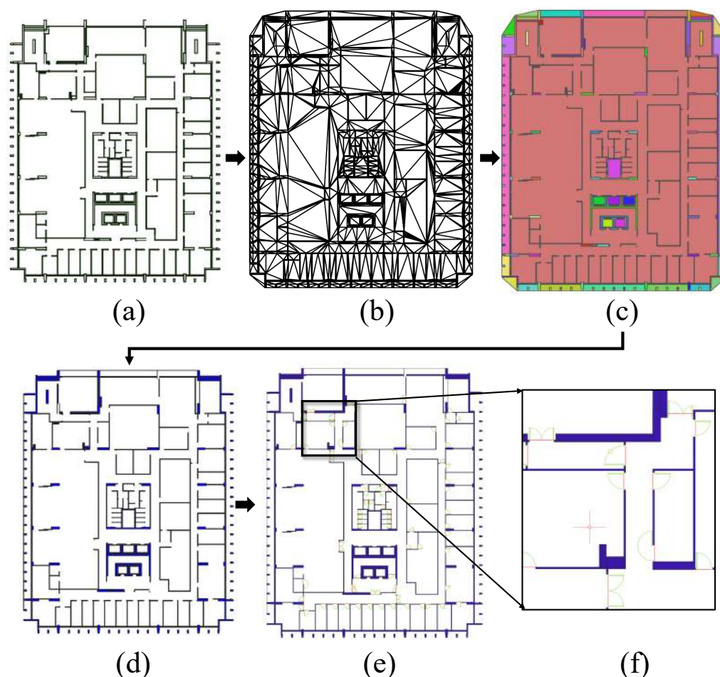
Figure 3. Polygonization of 2D story plan based on CAD drawings. (a) Filtered segments of vertical structures; (b) triangles by constraint triangularization; (c) merged polygons; (d) filtered and filled polygons of structures; (e) simplified door symbols connecting walls; (f) details of simplified doors, where the green lines are the original symbols and the red ones are simplified results.
